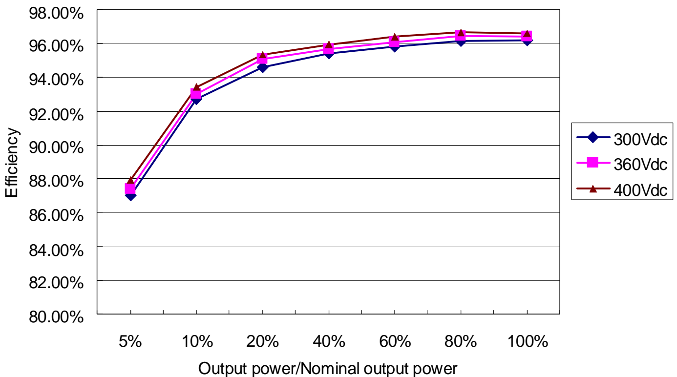
Efficiency curve
